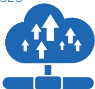
SERVER VIRTUALIZATION
